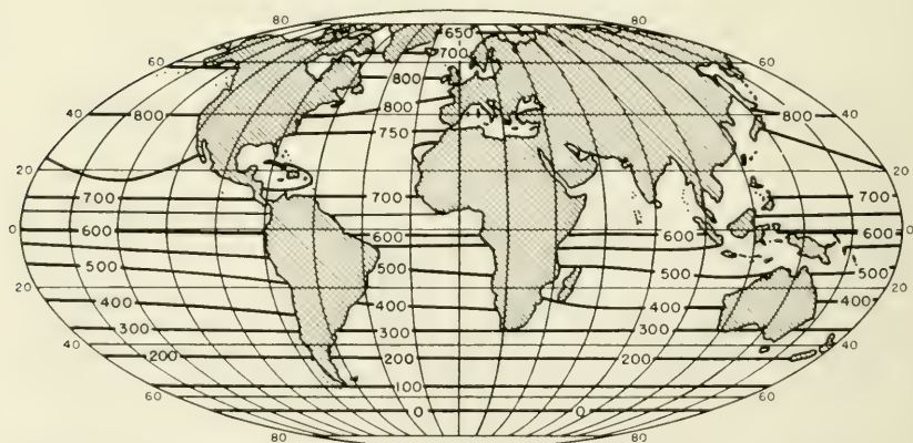
FIG. 6.4. Total solar radiation (g-cal/day/cm² of horizontal surface) on June 21 with cloudless sky. (Modified from Kimball, 1928.)
