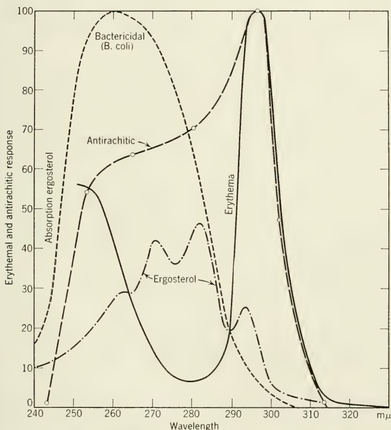
FIG. 6.25. Relation between wavelength in the ultraviolet region and the bactericidal, erythemic, and antirachitic effects of ultraviolet radiation, together with the absorption of ergosterol. (Coblentz, 1939, Copyright, J. Am. Medical Assoc.)
