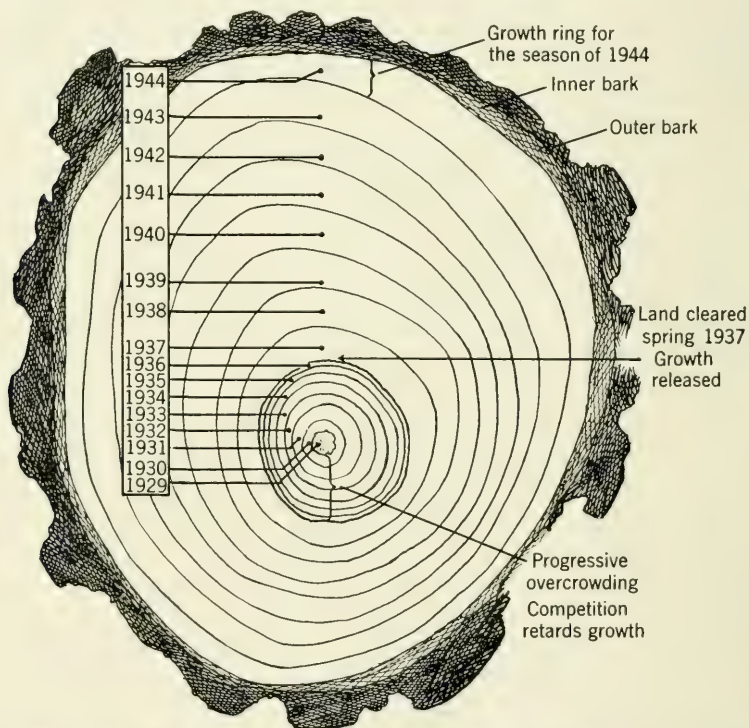
FIG. 9.3. Cross section of locust tree ( Robinia Pseudo-Acacia ), 17 cm in diameter, grown in Belmont, Mass., showing effects of early overcrowding and subsequent "release."
