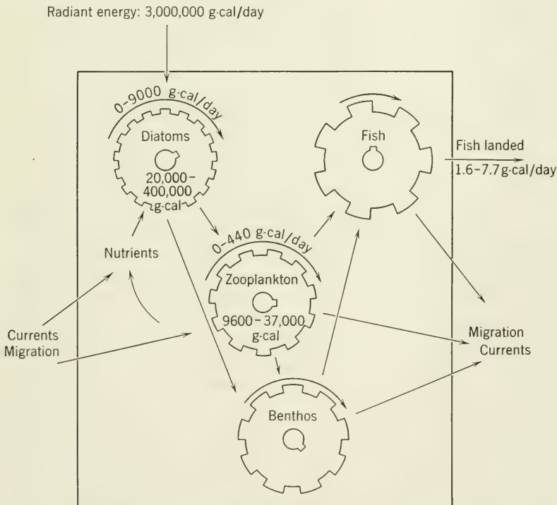
FIG. 13.12. Principal components and processes involved in production on Georges Bank, off Massachusetts. Values are averages for the whole bank per square meter of sea surface. Maximum and minimum values within the cogwheels are for the standing crop; those over the wheels are for net production rate.
