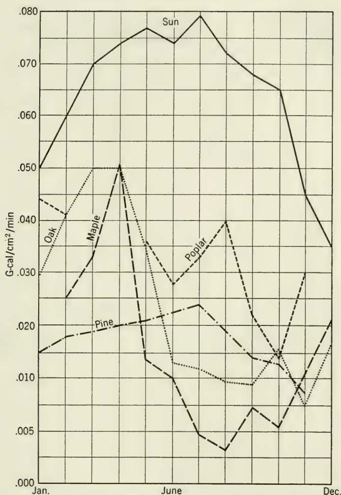
FIG. 6.2. Mean monthly maximum intensities of solar ultraviolet radiation (2900-4000Å) in forest communities of northern Indiana. (Strohecker, 1938.)
