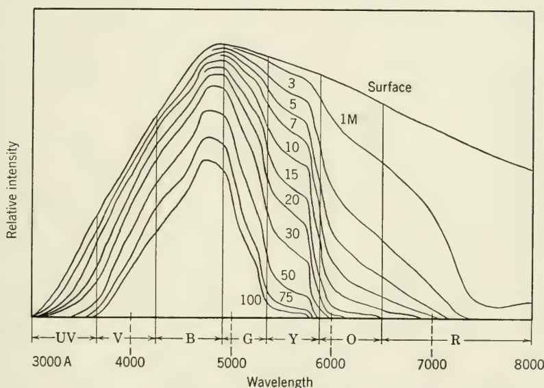
FIG. 6.6. The spectral distribution of solar energy at the earth's surface and after modification by passage through the indicated meters of pure water. Similar light conditions would be found in the clearest ocean and lake waters. (Clarke 1939, AAAS Publ. No. 10.)
