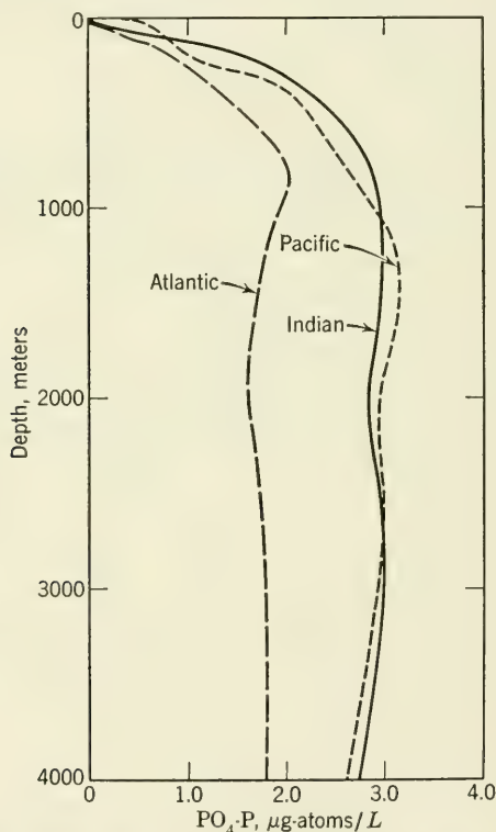
FIG. 8.8. Vertical distribution of phosphate in the Atlantic, Pacific, and Indian Oceans. (From The Oceans by Sverdrup et al., 1942, Copyright, Prentice-Hall, N. Y.)
