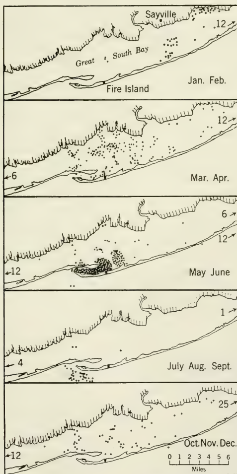
FIG. 5.9. Thermal migration of the winter flounder as revealed by the recapture, at the points indicated, of fish tagged and released in Great South Bay, Long Island.
