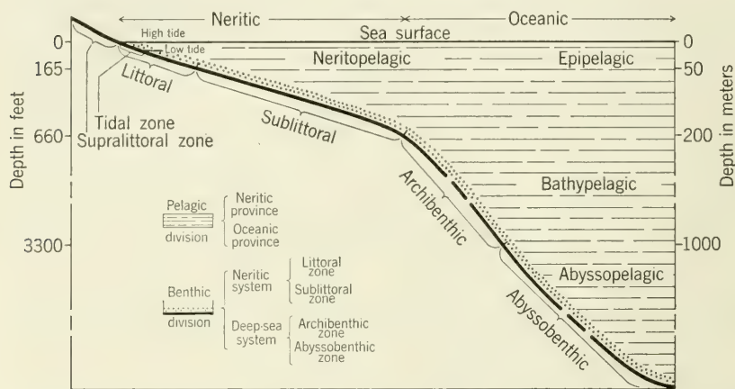
FIG. 2.4. The chief zones of the marine environment. The division between the neritic and oceanic provinces occurs at the edge of the continental shelf where depth is about 200 m. The lower limit of the archibenthic zone occurs between 800 and 1100 m. The littoral zone forms the upper part of the neritic benthic zone and usually receives strong wave and current action and sufficient light for plant growth. The depth of its lower limit is variable but is often in the neighborhood of 40 to 60 m. These divisions also apply in a general way to lakes. (Modified from The Oceans by Sverdrup et al., 1942, copyright Prentice-Hall, Inc., N. Y.)
