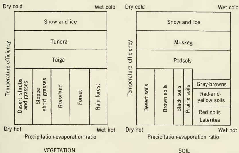
FIG. 5.22. Schematic representation of the interaction of temperature and moisture effectiveness in controlling the general distribution of vegetational life forms and soil groups in North America. (Modified from Thornthwaite, 1931.)
