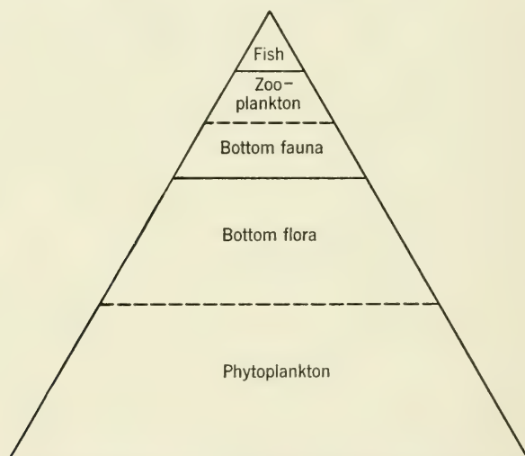
FIG. 13.2. Pyramid of biomasses as illustrated by the weight relationships of the various constituents of Weber Lake, Wisconsin. (Judy, 1943.)
