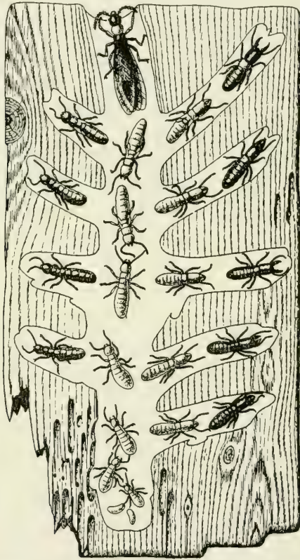
FIG. 9.10. The various forms of the termite Kalotermes flavicollis and their developmental origins. The eggs ( bottom ) hatch into young nymphs which after 5 to 7 molts reach the pseudergate stage (individual in center). From this stage the termite can change into a winged reproductive ( top ) by way of two wing-padded nymphs. At intermediate stages environmental influences may cause the nymphs to change into supplementary reproductives ( left ) or, by way of soldier nymphs, into soldiers ( right ). Most of the nymphs do not differentiate and these function as workers. All these stages are present in the termite colony, and their activities are integrated in its maintenance. (Lüscher, 1953, Sci. American , drawing by E. Mose.)
