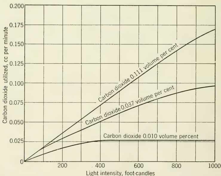
FIG. 7.8. Relation between rate of photosynthesis of wheat plants and light intensity at normal atmospheric, at decreased and at increased concentrations of carbon dioxide. (From Meyer and Anderson, 1939, after Hoover et al., Smithsonian Misc. Coll. , 1933.)
