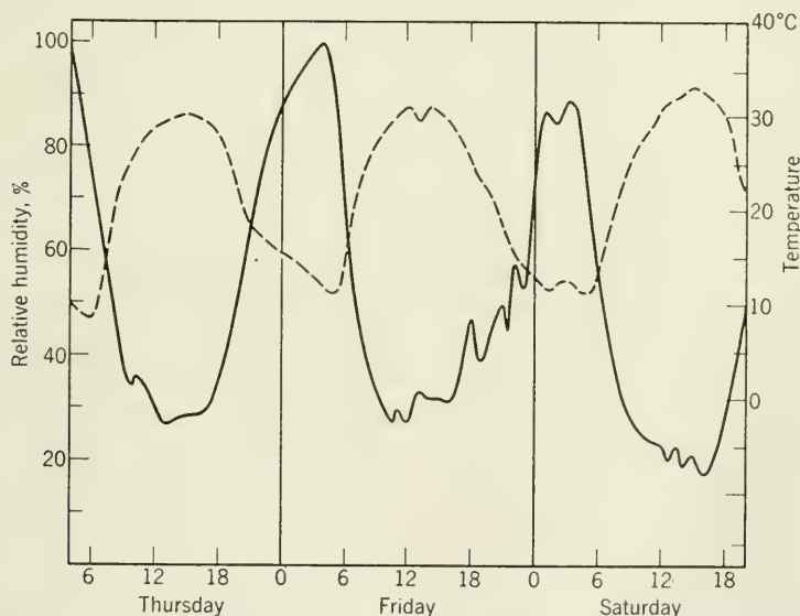
FIG. 4.11. Hygrothermograph record of temperature ( broken line ) and relative humidity ( solid line ) in the short-grass plains of central United States during 3 days in early July. (By permission from Plant Ecology by Weaver and Clements, 1938, McGraw-Hill Book Co.)
