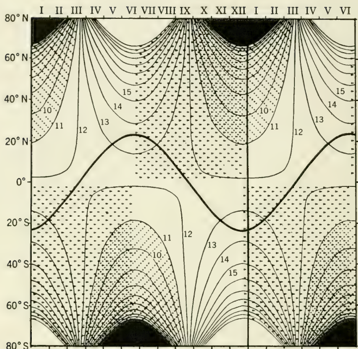
FIG. 6.3. Variation in length of day at the indicated latitudes during the indicated months. Arrowheads indicate periods of decreasing daylength. The heavy line shows the course of zenith sun (Baker, 1938.)
