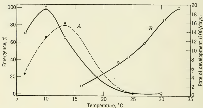
FIG. 5.16. The influence of temperature on (A) diapause development and (B) post-diapause morphogenesis in the embryo of the grasshopper, Austroicetes cruciata . Solid line: eggs from South Australia; broken line: eggs from West Australia.
