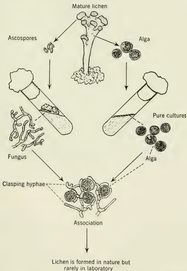
FIG. 10.1. Diagram illustrating the symbiotic partnership represented by the lichen Cladonia cristatella and its separation in the laboratory into algal and fungal components. When the components are recombined in the laboratory, the typical morphology of the lichen is not developed, evidently because of the lack of certain environmental conditions found in nature. (Burkholder, 1952, Copyright Baitsell's Science in Progress , Yale University Press.)
